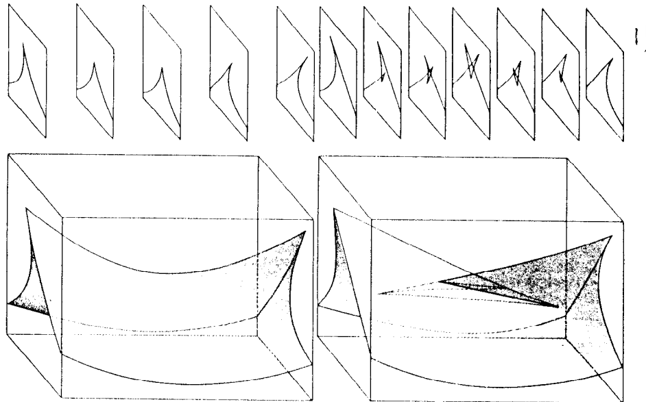
BUTTERFLY
