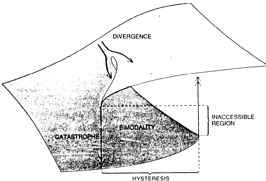
FIVE PROPERTIES characterize phenomena that can be described by the cusp catastrophe. The behavior is always bimodal in some part of its range, and sudden jumps are observed between one mode of behavior and the other. The jump from the top sheet of the behavior surface to the bottom sheet does not take place at the same position as the jump from the bottom sheet to the top one, an effect called hysteresis. Between the top and bottom sheets there is an inaccessible zone on the behavior axis; the middle sheet, representing least likely behavior, has been omitted for clarity. Finally, the cusp catastrophe implies the possibility of divergent behavior.
