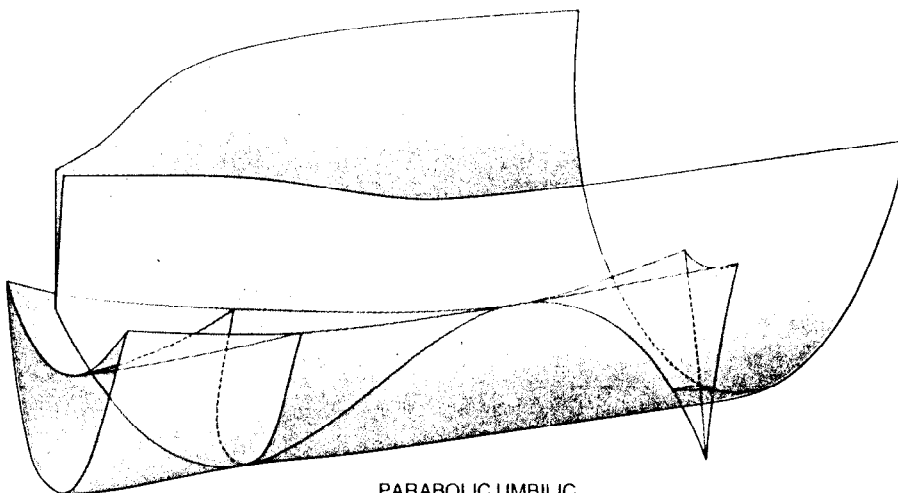
PARABOLIC UMBILIC
